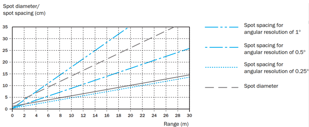
Figure 8 spot spacing in cm versus range in m for ( 0.25^\circ , 0.5^\circ or 1^\circ ) angular resolution
