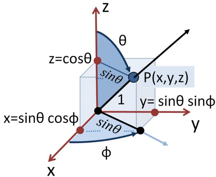
Figure 2 Relation between Cartesian and Polar co-ordinates
