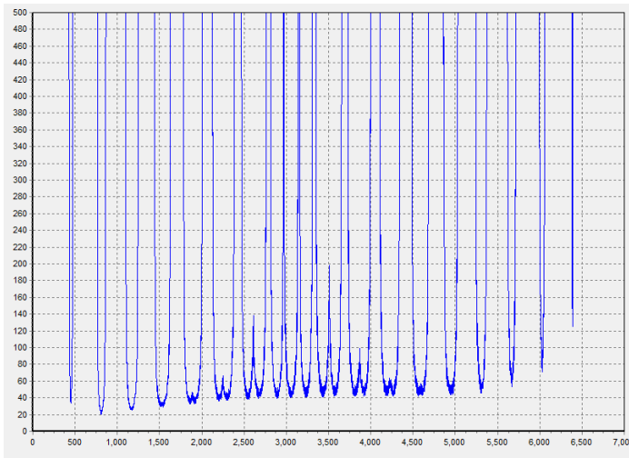
Figure 15 Simulated range sensor data versus time based on collected Field sea trial logged data during turning in a full circle
