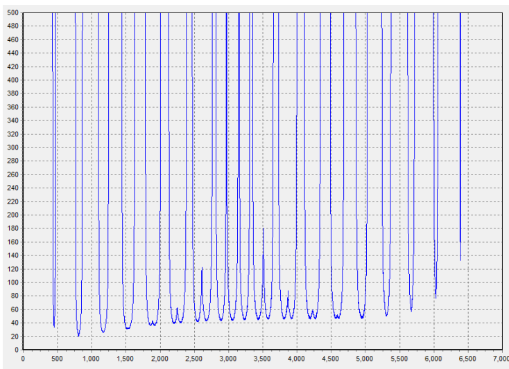
Figure 14 Real range sensor data versus time based on collected Field sea trial logged data during turning in a full circle
