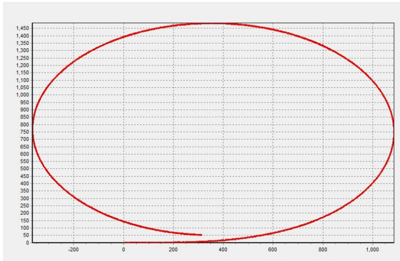
Figure 11 Field sea trial logged data during turning in a full circle (ship course)
