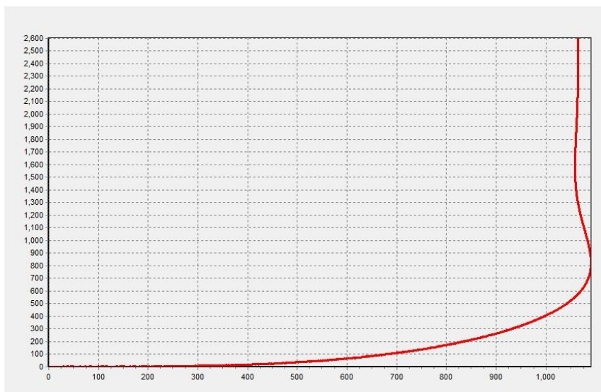
Figure 17 Field sea trial logged data during changing course from 0° to 90° (ship course)
