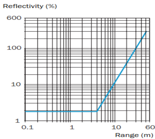
Figure 9 relation between reflectivity and detection range
