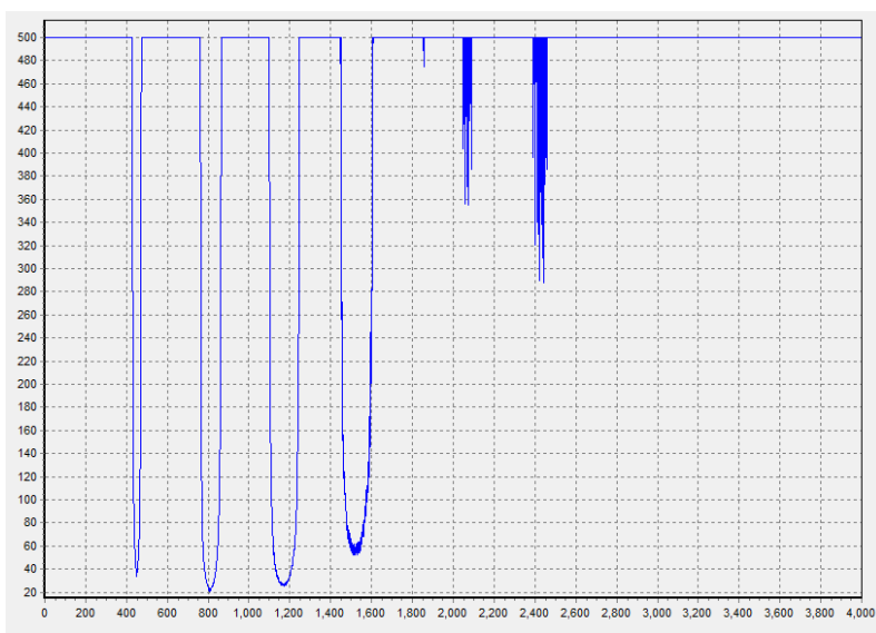
Figure 20 Simulated range sensor data versus time based on collected Field sea trial logged data during changing course from 0° to 90°
